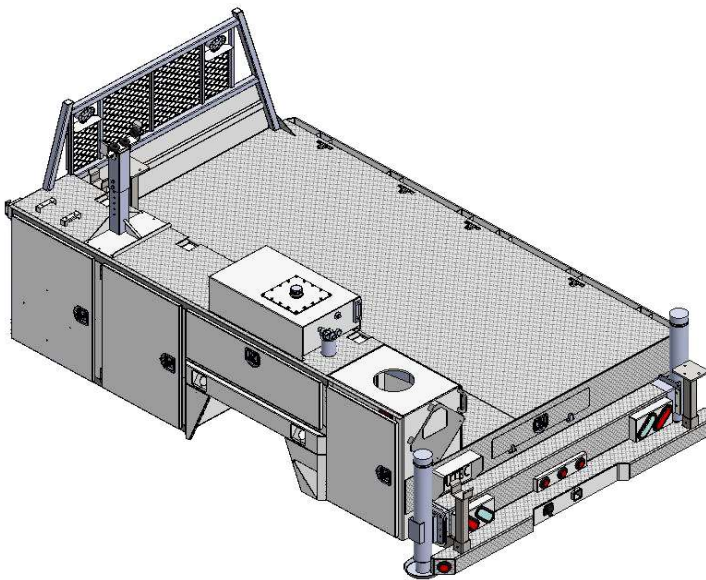
DSD 84 LP CRANE BODY WITH LP FUEL SUPPLY TANK UNDER PASSENGER FRONT SIDE
